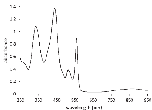
Figure 6. UV–vis–NIR absorption spectrum of [(C=C)TTP][OTf]_2 in CH_2Cl_2 , showing \lambda_{max} values of 335, 439, 512, 559, and 864 nm.
